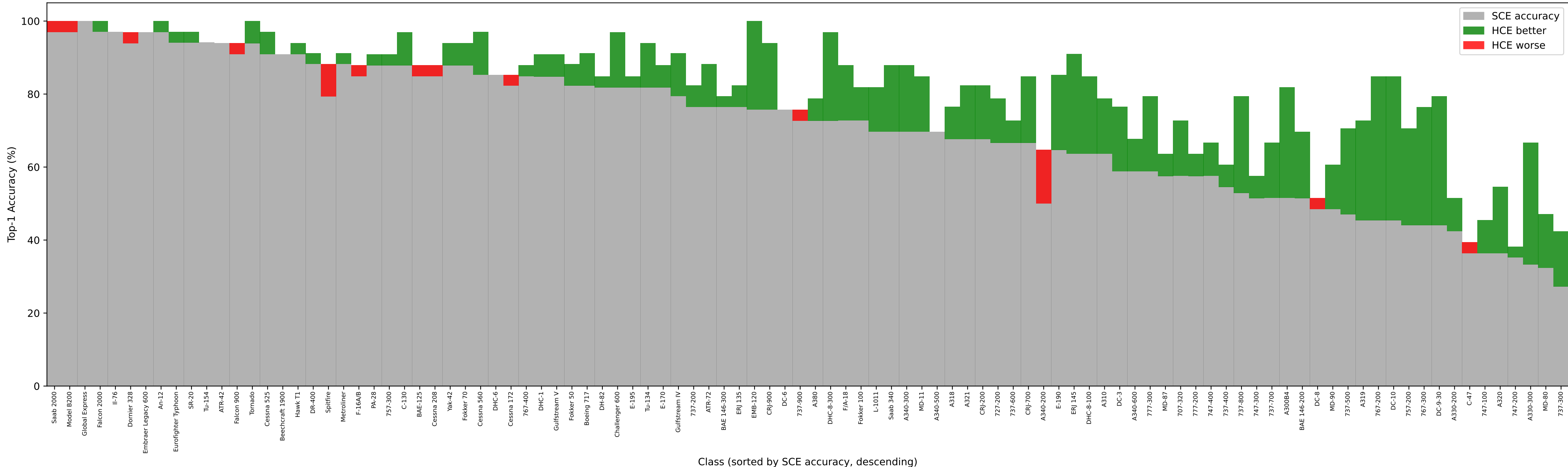
ResNet-50 — Per-variant accuracy: SCE vs HCE
